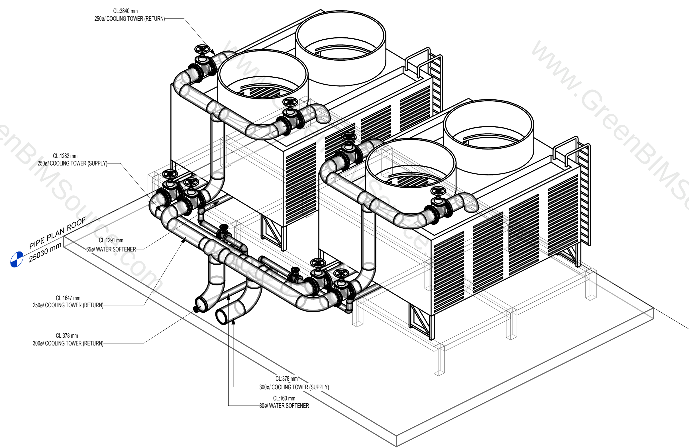
8 3D - COOLLING TOWER
