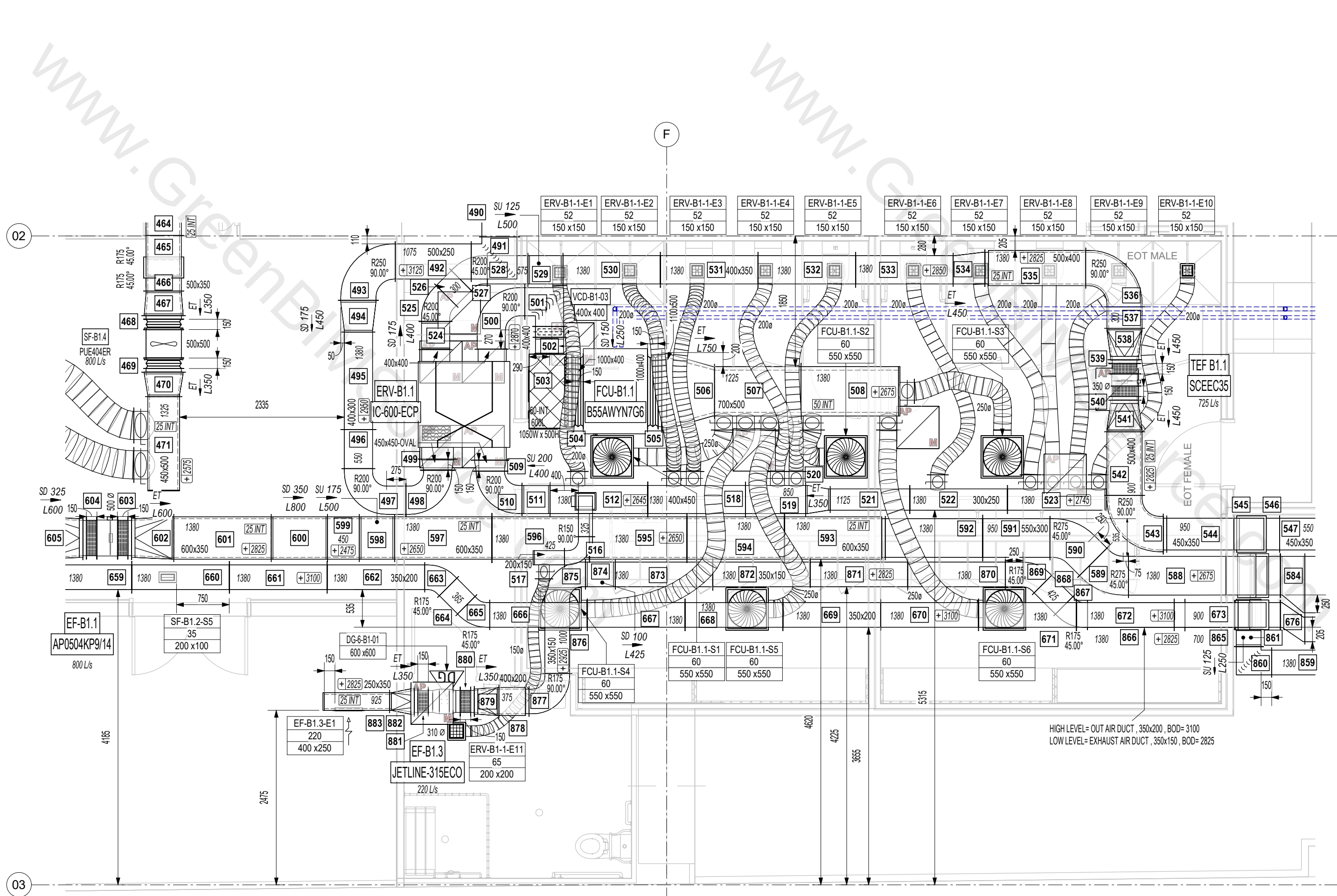
1 BASEMENT 1 MECHANICAL LAYOUT - Callout 1 1:50
