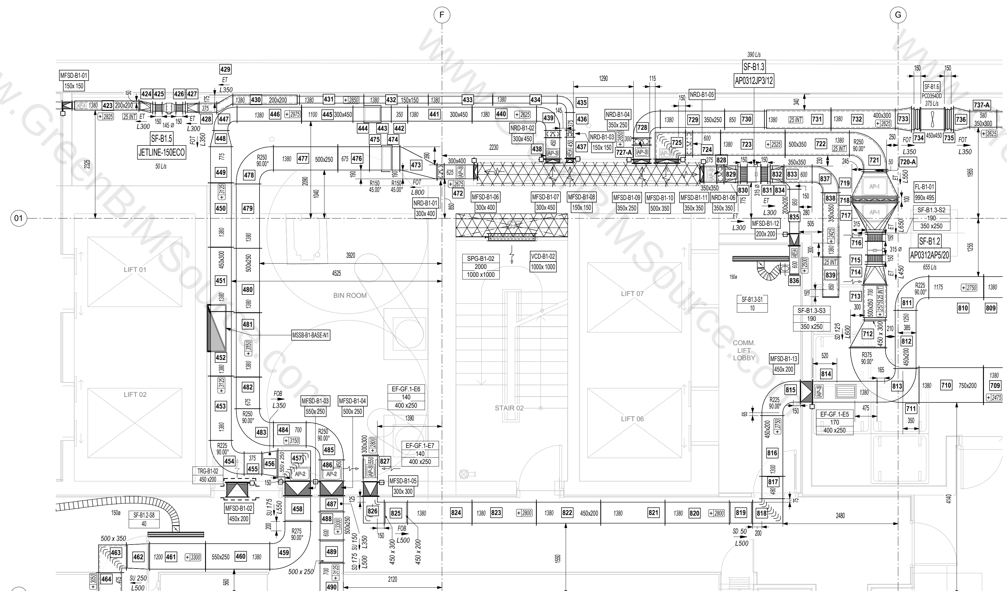
2 BASEMENT 1 MECHANICAL LAYOUT - Callout 2 1:50
