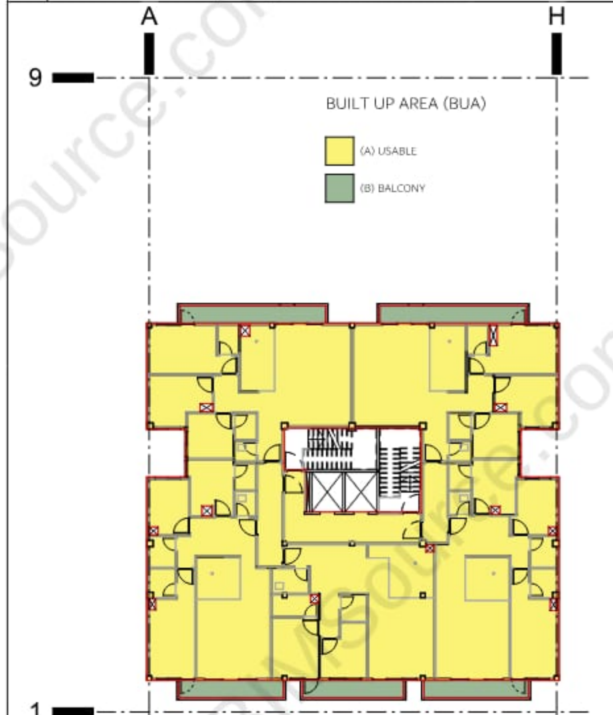
04 BUA-SECOND TO FOURTH FLOOR (1 : 250)
